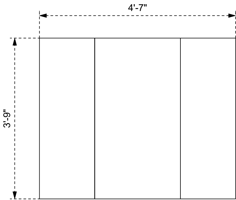
Top Plan
