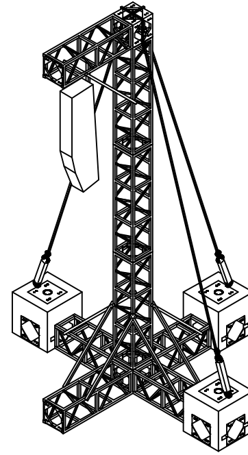
Iso View
