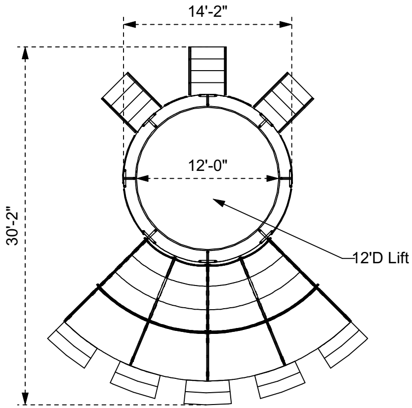
Top Plan
