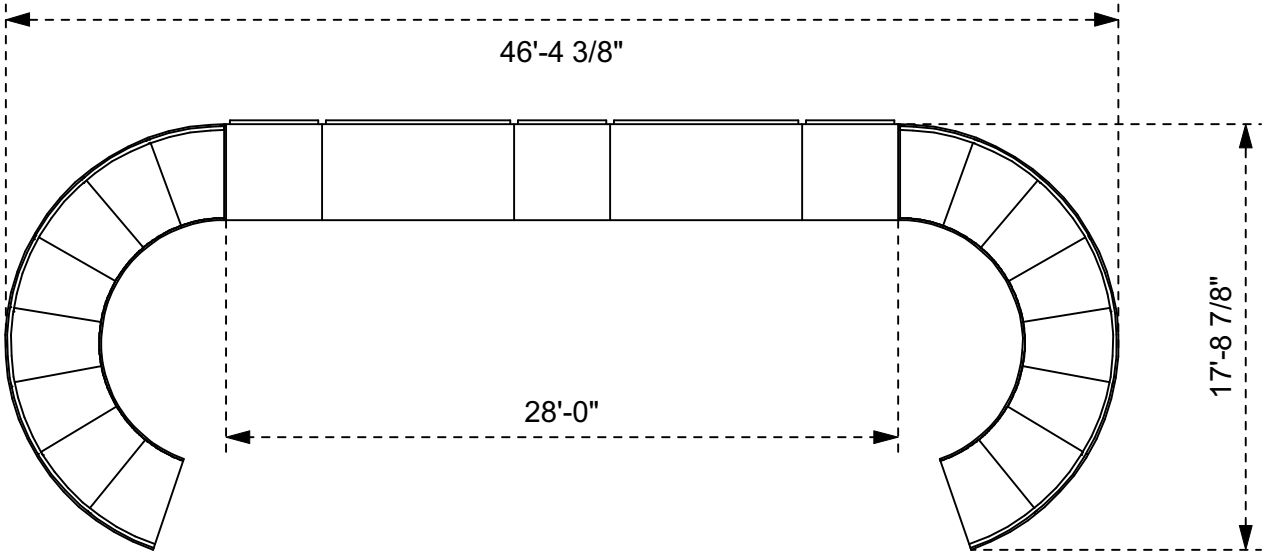
Top Plan
